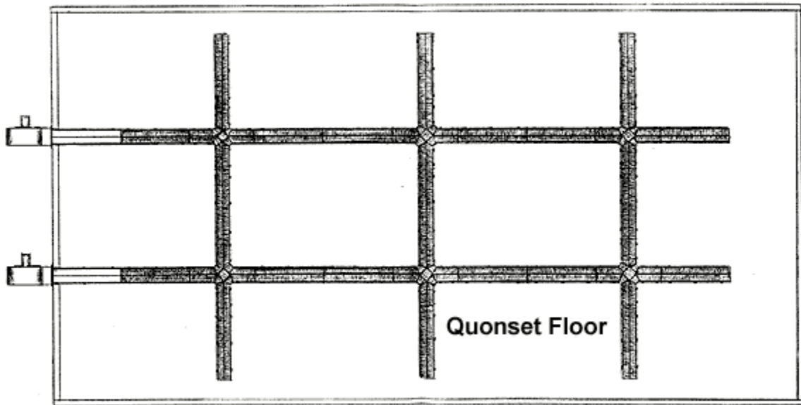
Layout with fans at the end
